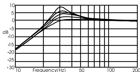
FIG. 4 VARIABLE BOOST
