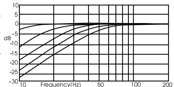
FIG. 3 VARIABLE HIGH PASS
