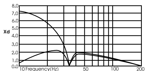
FIG. 5 LIMITED EXCURSION
